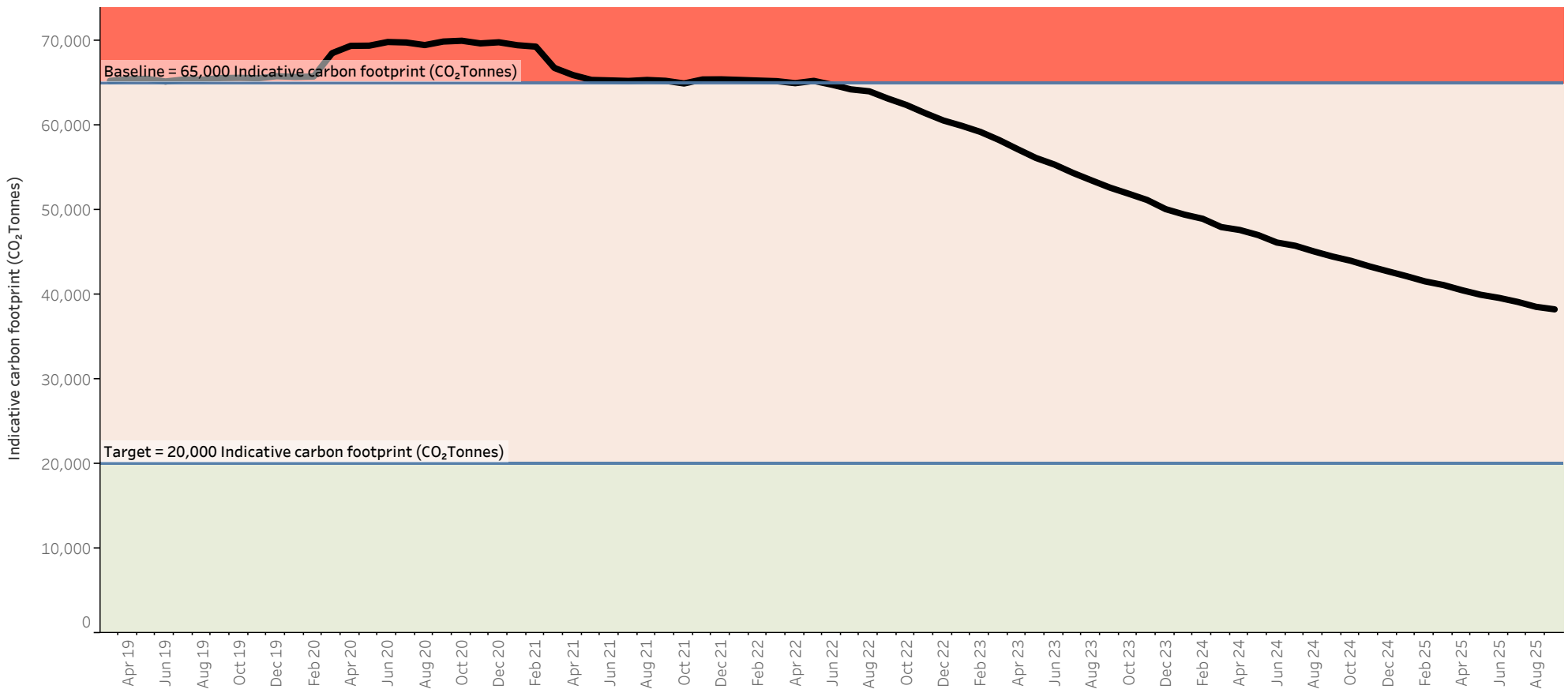
Figure 2. The indicative annual carbon footprint of all inhalers issued within primary care in Wales – from April 2019 to September 2025
