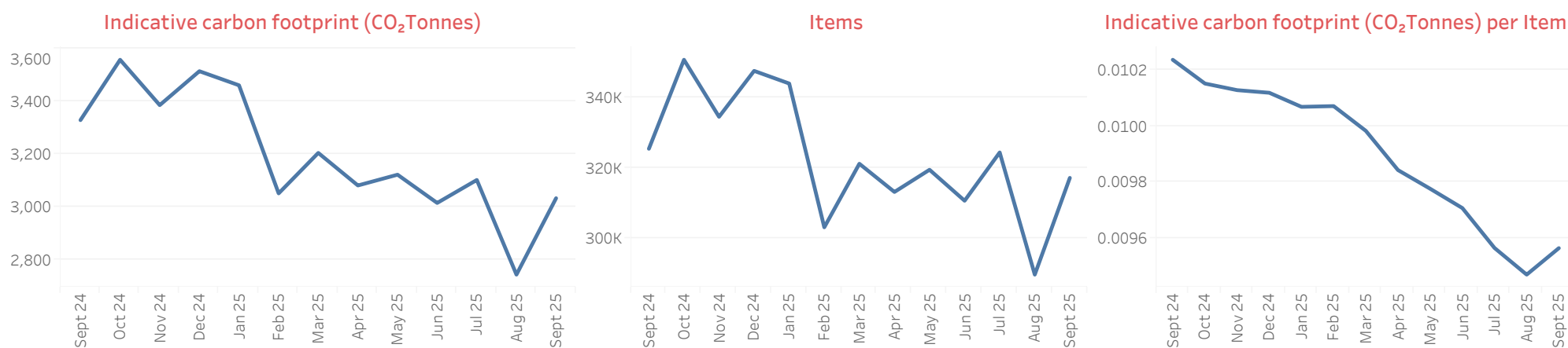
Figure 1. The indicative carbon footprint, number of inhaler items, and indicative carbon footprint per item issued within primary care in Wales September 2024 to September 2025
