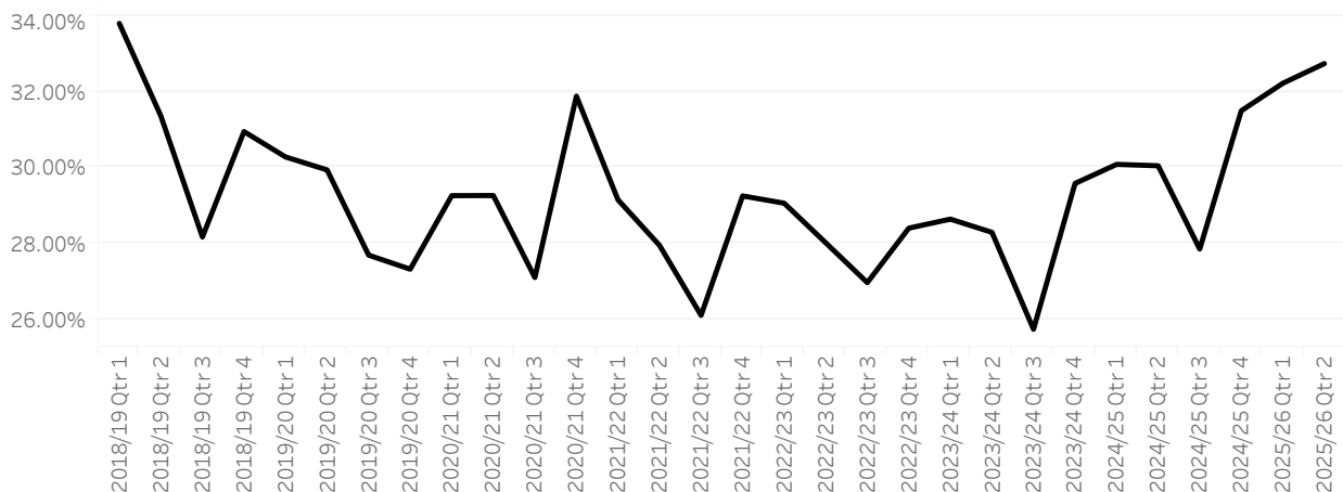
Figure 7. Combined DPI and SMI percentage of total inhaler quantity issued in secondary care from April 2018 to September 2025
