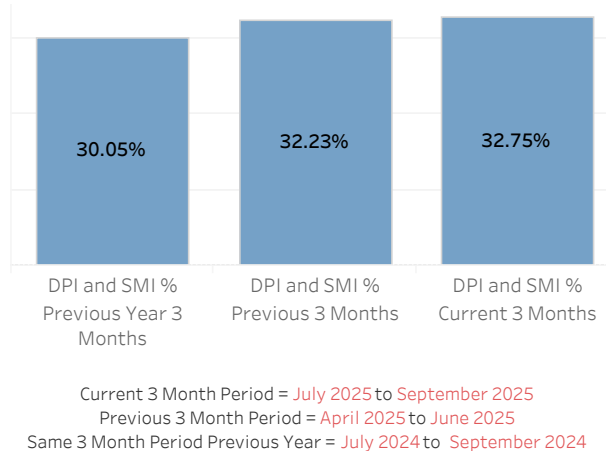
Figure 8. Combined DPI and SMI percentage of total inhaler quantity issued in secondary care
