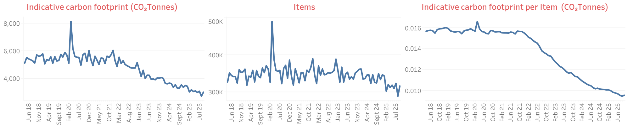
Figure 4. The indicative carbon footprint, number of inhaler items issued, and indicative carbon footprint per item, changes between April 2018 to September 2025, within primary care in Wales from April 2018 to September 2025
