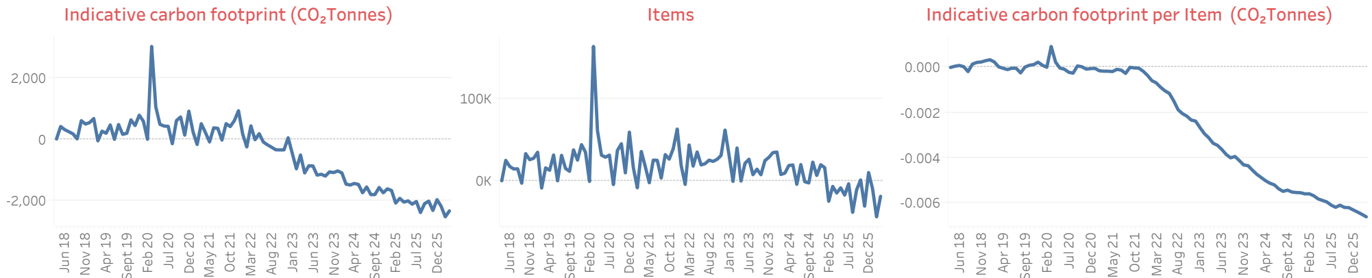
Figure 4. The indicative carbon footprint, number of inhaler items issued, and indicative carbon footprint per item, changes between April 2018 to March 2026, within primary care in Wales from April 2018 to March 2026
