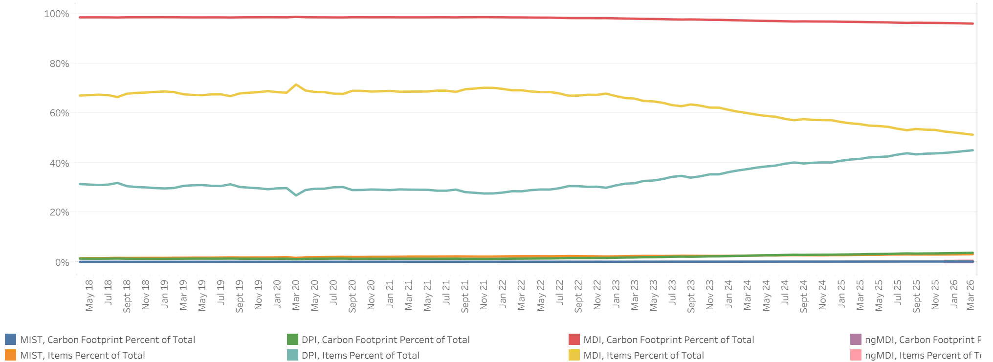
Figure 5. Item number and carbon footprint associated with the use of different inhaler types as a percentage of all inhalers issued within primary care in Wales – from April 2018 to March 2026
