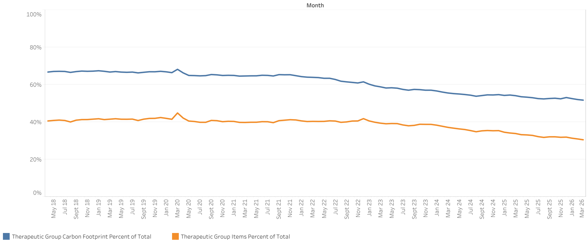
Figure 6. Item number and carbon footprint of SABA inhalers as a percentage of all inhalers issued within primary care in Wales – from April 2018 to March 2026
