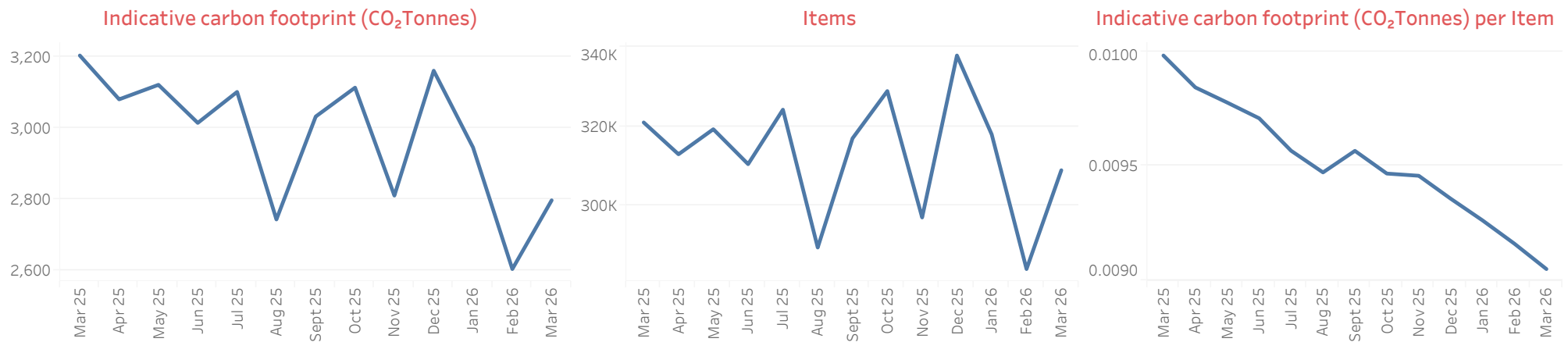
Figure 1. The indicative carbon footprint, number of inhaler items, and indicative carbon footprint per item issued within primary care in Wales March 2025 to March 2026
