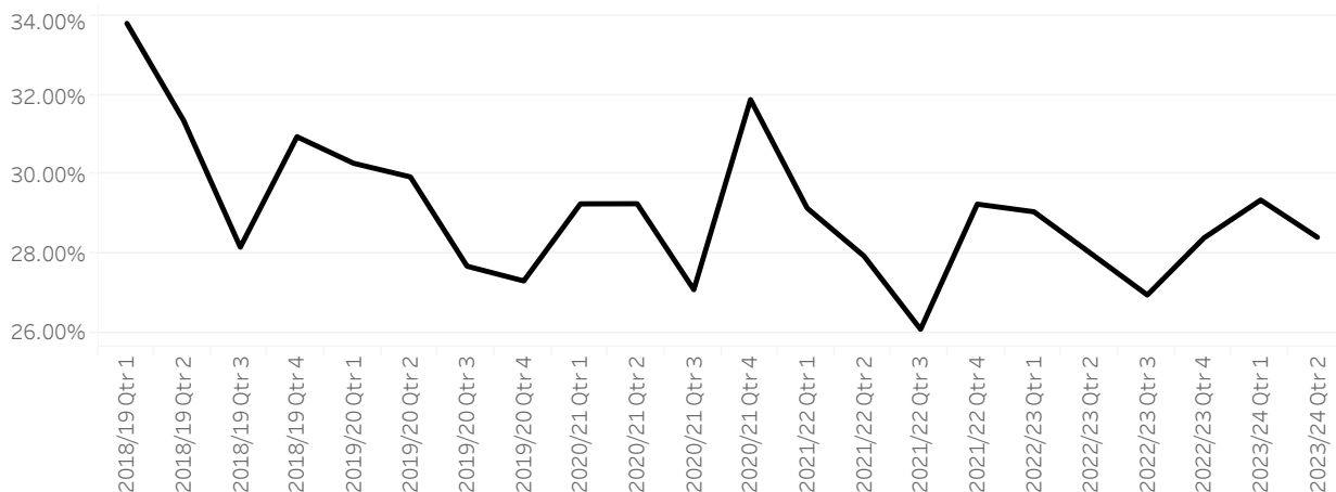
Figure 7. Combined DPI and SMI percentage of total inhaler quantity issued in secondary care from April 2018 to September 2023
