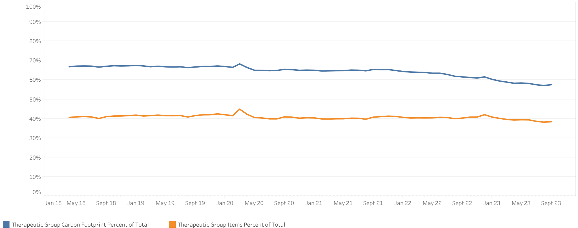
Figure 6. Item number and carbon footprint of SABA inhalers as a percentage of all inhalers issued within primary care in Wales – from April 2018 to September 2023
