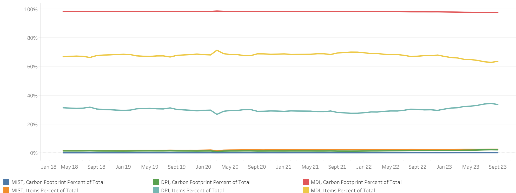
Figure 5. Item number and carbon footprint associated with the use of different inhaler types as a percentage of all inhalers issued within primary care in Wales – from April 2018 to September 2023
