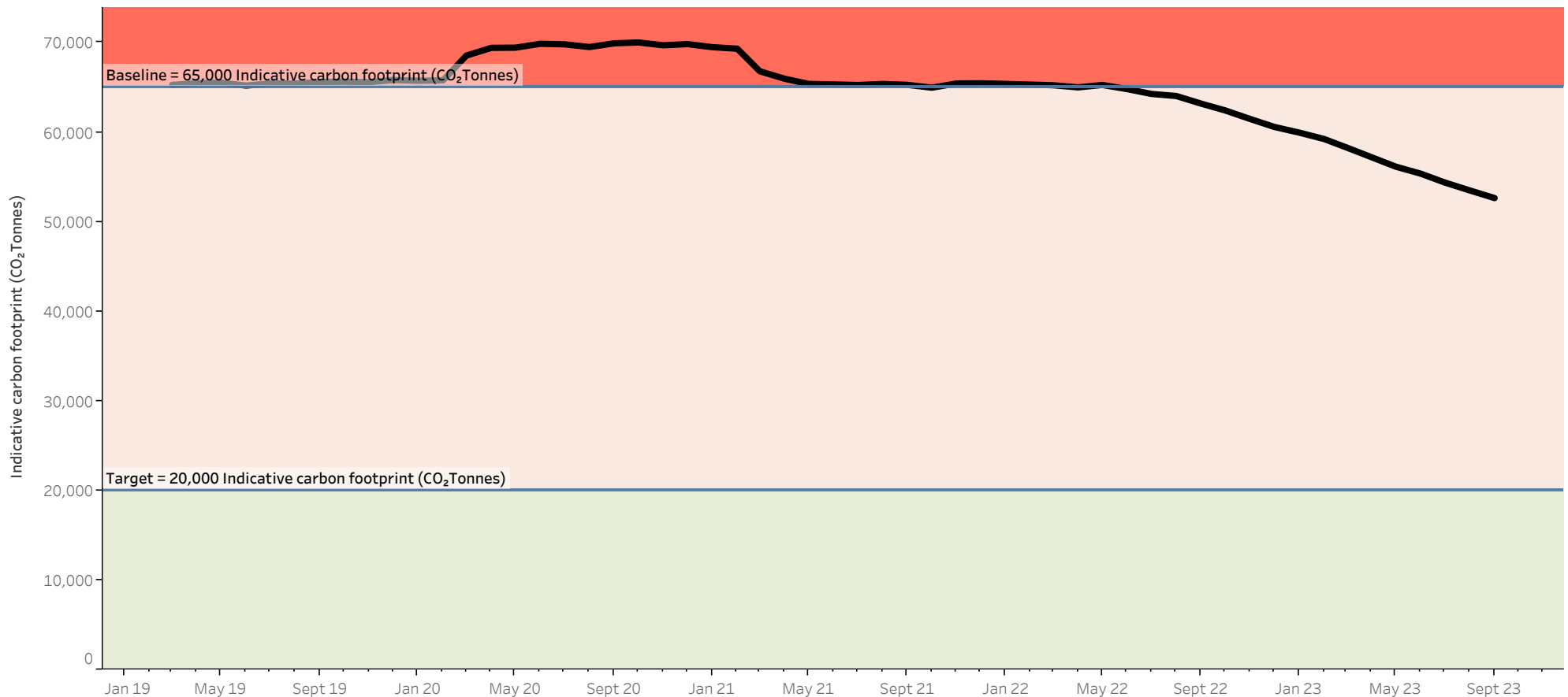
Figure 2. The indicative annual carbon footprint of all inhalers issued within primary care in Wales – from April 2019 to September 2023
