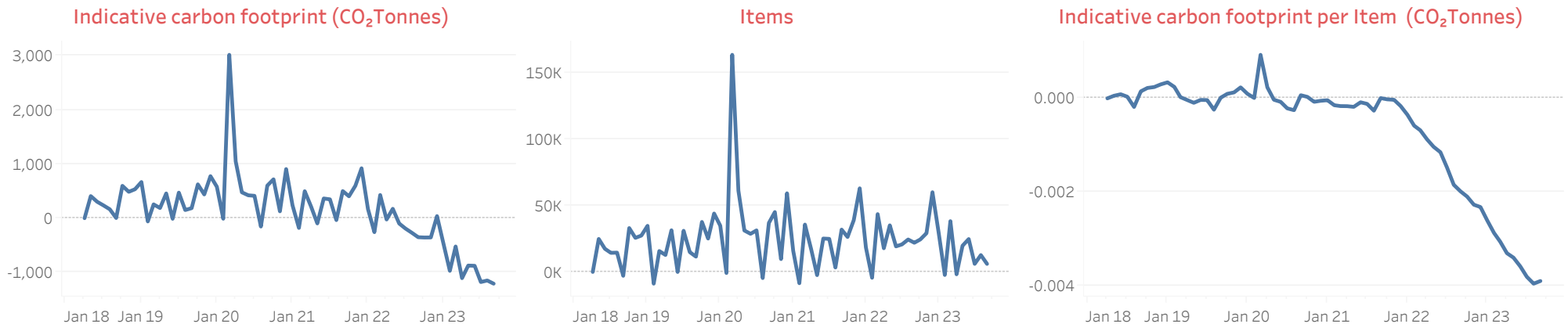
Figure 4. The indicative carbon footprint, number of inhaler items issued, and indicative carbon footprint per item, changes between April 2018 to September 2023, within primary care in Wales from April 2018 to September 2023
