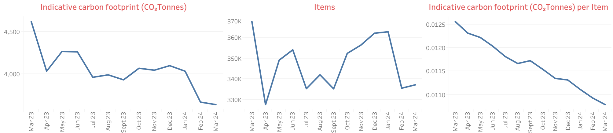
Figure 1. The indicative carbon footprint, number of inhaler items, and indicative carbon footprint per item issued within primary care in Wales March 2023 to March 2024
