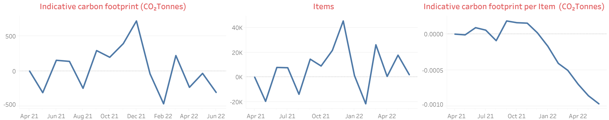
Figure 3. The indicative carbon footprint, number of inhaler items, and indicative carbon footprint per item issued within primary care in Wales from April 2021 to June 2022
