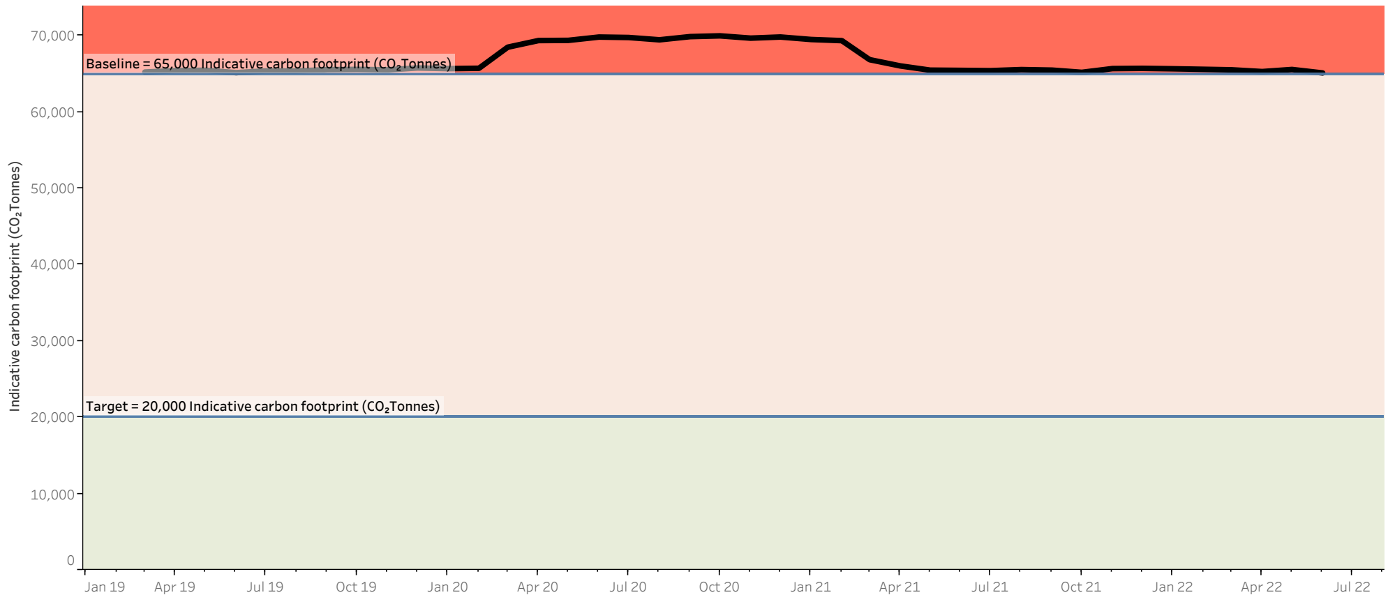
Figure 1. The indicative annual carbon footprint of all inhalers issued within primary care in Wales – data to June 2022
