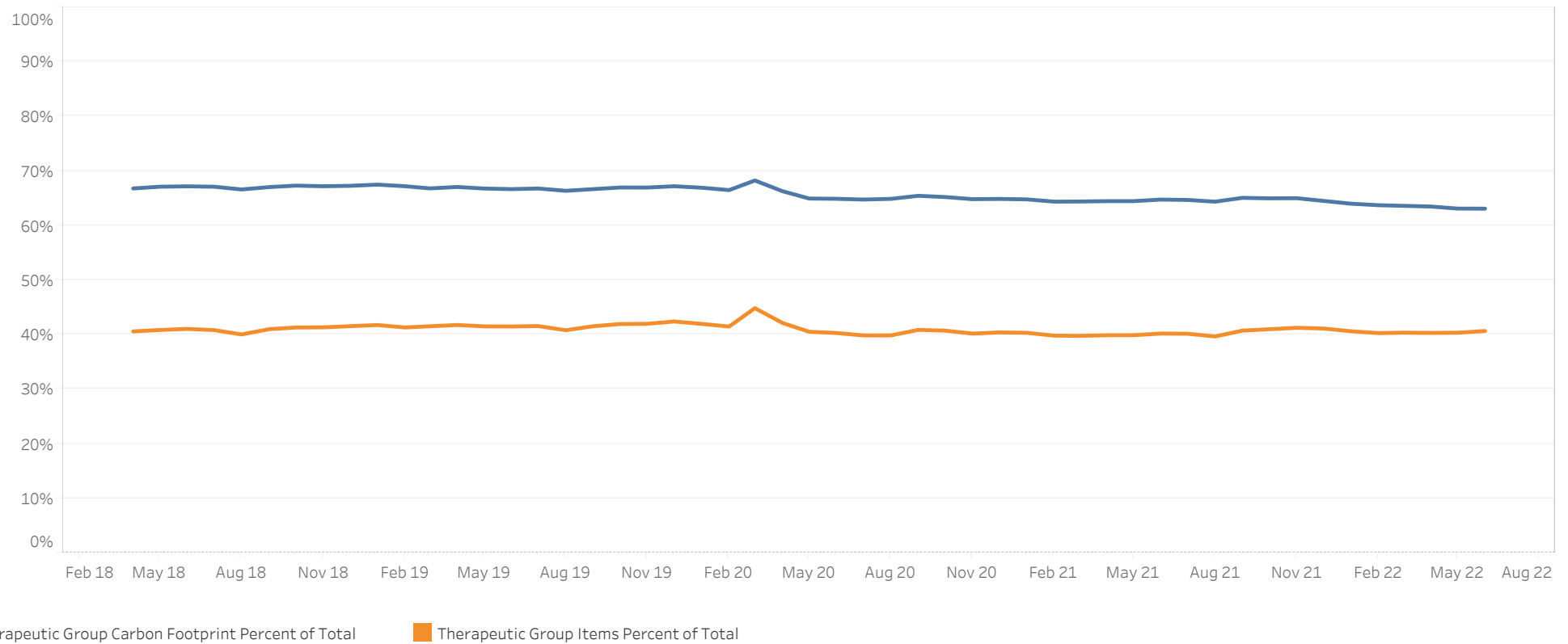
Figure 5. Item number and carbon footprint of SABA inhalers as a percentage of all inhalers issued within primary care in Wales – data to June 2022
