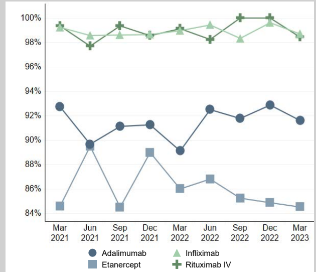
Biosimilar usage in Cardiff and Vale (as a % of total biologic) - Quarterly trend up to March 2023
